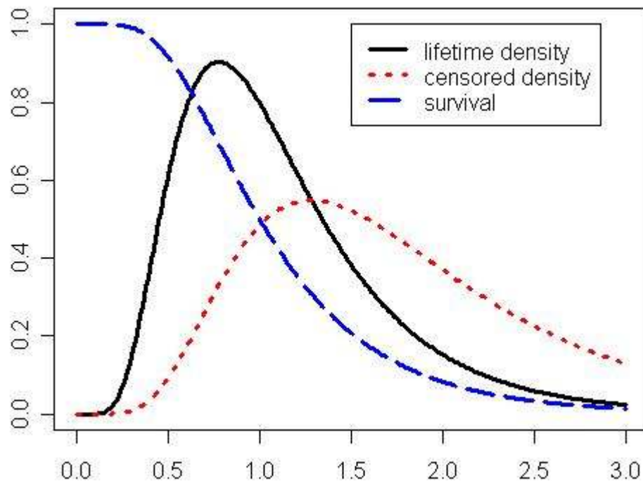
FIG 2. Lifetime and censored Weibull densities considered in the simulations with a plot of the survival function also included.
