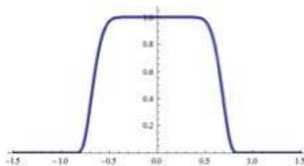
FIG 1. Infinitely differentiable flat-top function (8) with parameters b = 1 and c = .05 .
